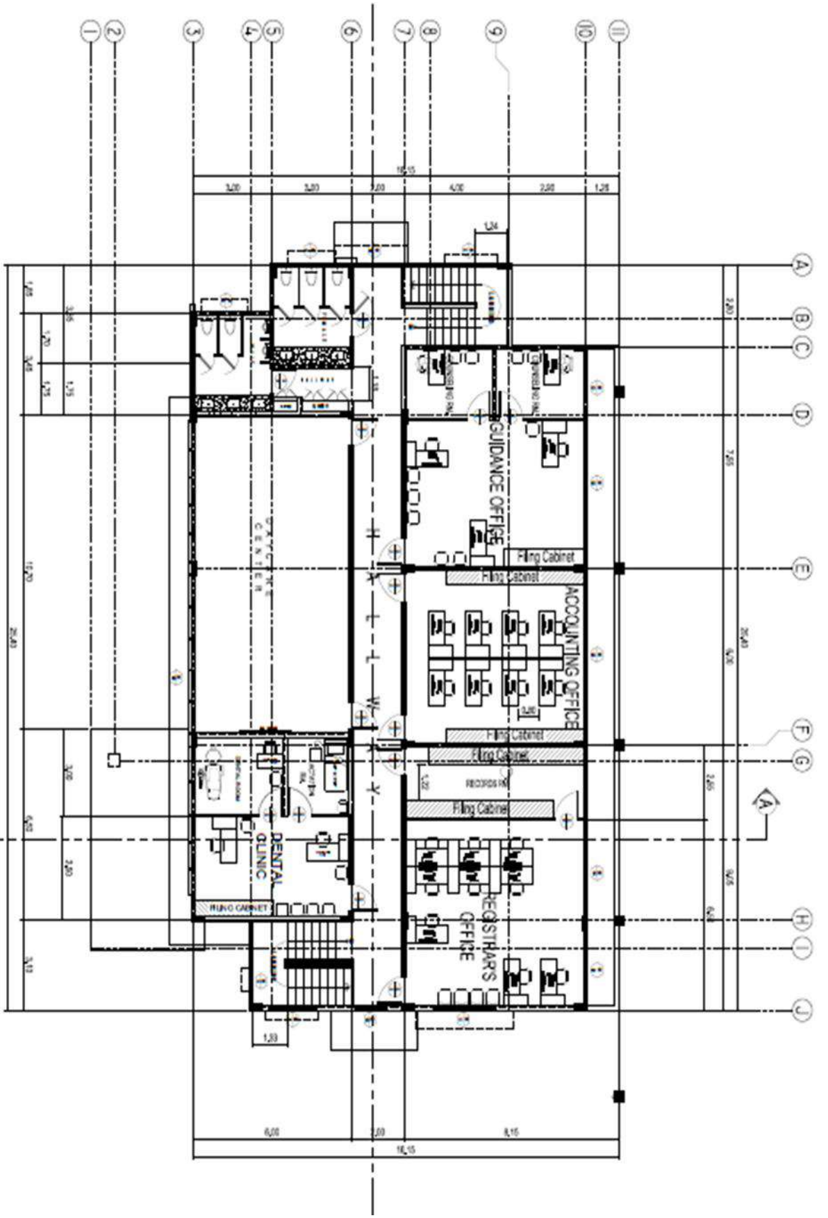
1 SECOND FLOOR PLAN SCALE 1/8" = 1'-0" 1/8" = 1'-0"
